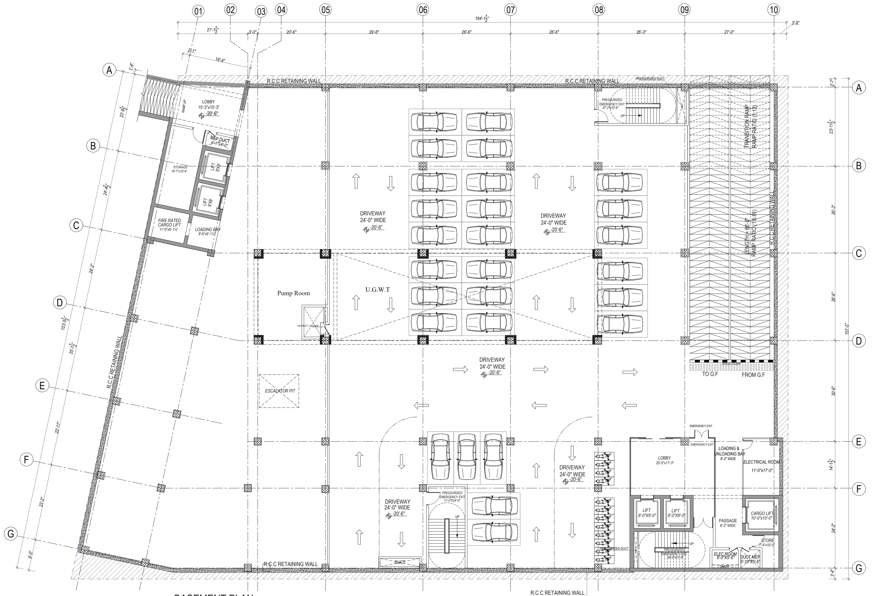
BASEMENT PLAN
